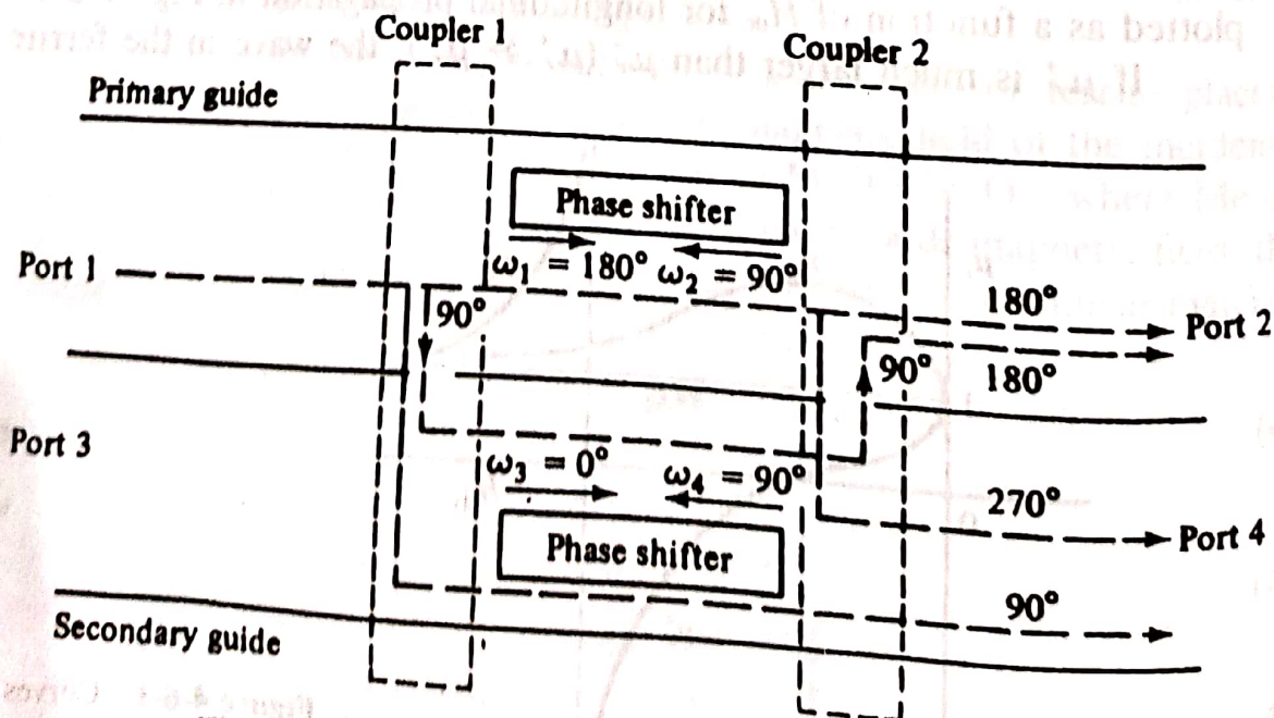
Figure 4-6-3 Schematic diagram of four-port circulator.
