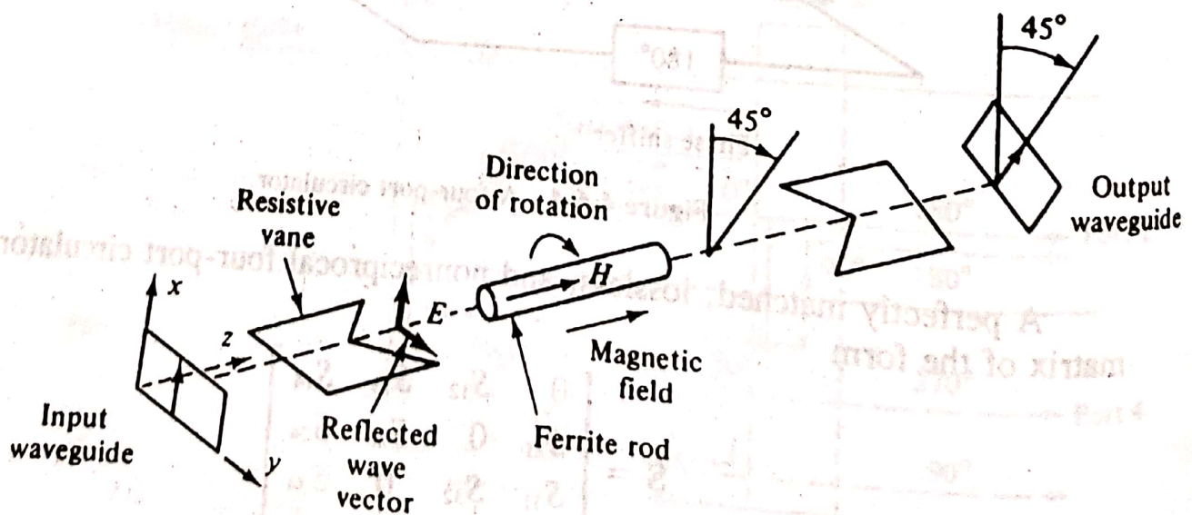
Figure 4-6-5 Faraday-rotation isolator.
