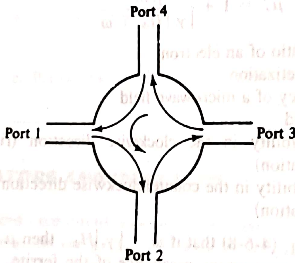
Figure 4-6-2 The symbol of a circulator.
